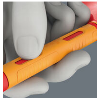
The recesses in the fast-rotating sleeve allow resistance to be generated by finger force. This allows the ratchet mechanism to be used even at low resistance of the screw.
